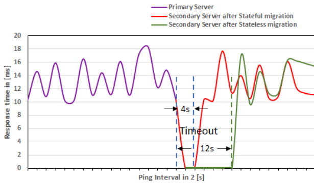
Fig. 4: UE Service Downtime
