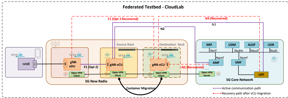
Fig. 3: Demo Setup
