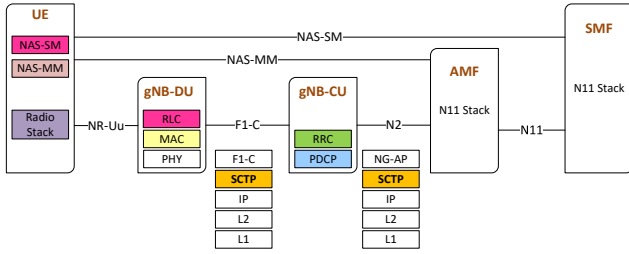
Fig. 1: 5G Control Plane Protocol Stack
