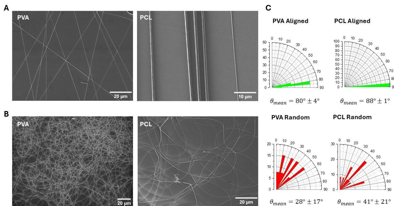
Figure 1. SEM images of A) Aligned PVA and PCL fibers, B) Random PVA and PCL fibers, C) Alignment degrees diagrams of each sample and mean angles.
