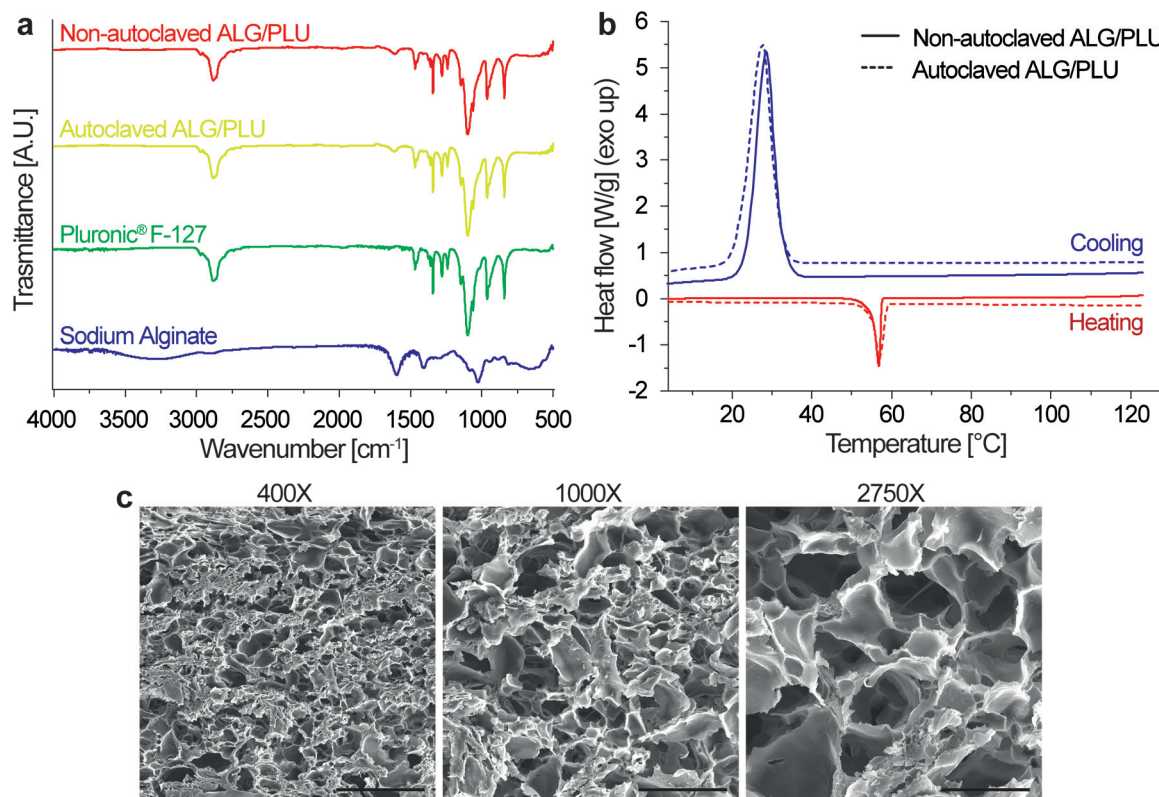
Fig. 3 (a) FT-IR spectra of ALG/PLU-based bioinks before and after autoclave, Pluronic® F-127, and sodium alginate. (b) DSC curves of autoclaved and non-autoclaved ALG/PLU-based bioinks; for both conditions, only the second heating curve and the cooling curve are shown. ALG/PLU: alginate/Pluronic-based bioink. (c) Representative SEM images at different magnifications showing the hydrogel internal section of non-doped printed structures, in the absence of cells. Scale bar: 200, 80, and 30 \mu\text{m} for 400 \times , 1000 \times , and 2750 \times magnification, respectively.
