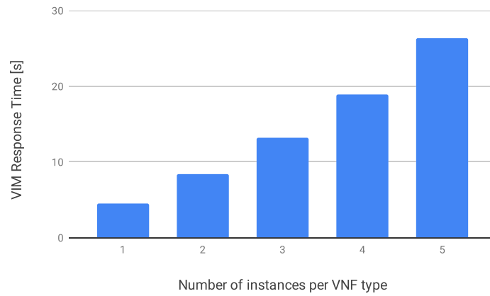
Fig. 9. Response time at the VIM for service chain deployment as a function of the number of VNF instances per VNF type, for the case of a chain size of 4 VNFs.
