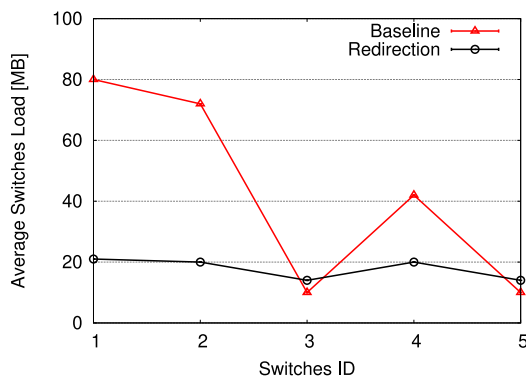
Fig. 14. Impact of the load-balancing algorithm on the switches load.
