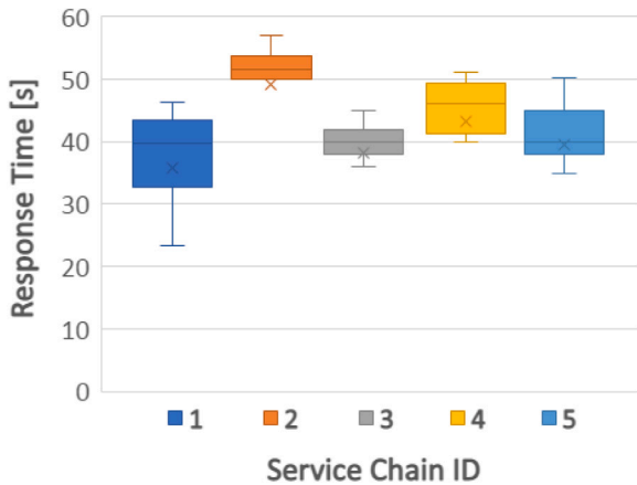
Fig. 11. Response time of path service chains.
