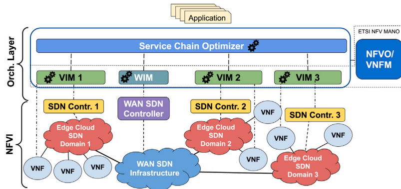
Fig. 2. Orchestration system architecture for latency-aware and adaptive service chaining orchestration.
