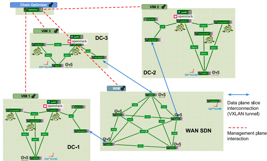
Fig. 5. Experiment Deployment on the Virtual Wall testbed from the Fed4FIRE experimentation platform.
