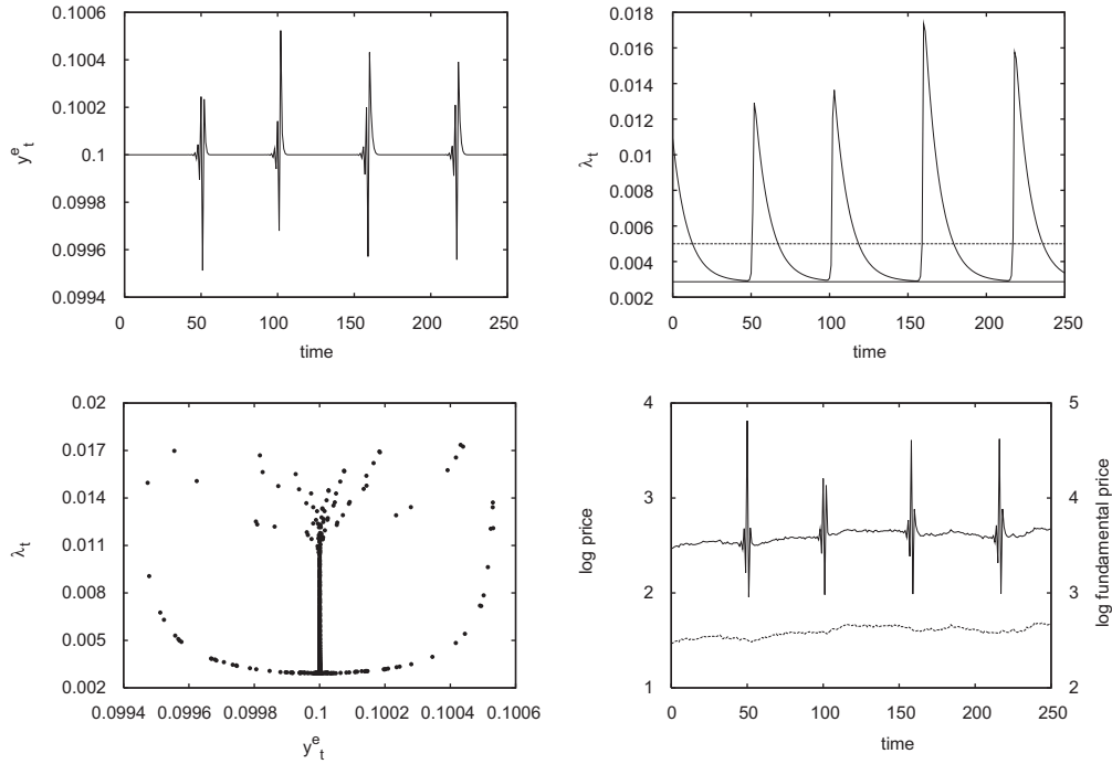
Fig. 2. Top panels: time series for the expected dividend yield y_t^e (left panel) and the fraction of informed agents \lambda_t (right panel) from (28) to (29). In the top right panel the dotted line corresponds to \bar{\lambda} in (31) (the critical stability border), whereas the solid line corresponds to the steady state \lambda^* in (32). The bottom left panel shows the state space representation (y_t^e, \lambda_t) . In the bottom right panel, the log price dynamics derived from the dynamics of y_t^e and \lambda_t is shown. Fundamental prices are given by the dotted line and realized prices by the continuous line. Notice that the two price series levels should be read using two different scales. The left scale gives the value of log prices, whereas the right scale gives the value of fundamental log prices. The dividend process is characterized by \sigma_\eta = 0.02 . Parameter values: \alpha = 0.99 , c = 0.1 , \rho = 1 (so that k = \rho/c = 10 ), r = 0.1 , g = 0 and \delta = 0.000575 .
