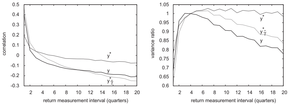
Fig. 7. Left panel: autocorrelation of the log return time series for a typical run of our model (35)–(37). Right panel: variance test of log lagged returns. v(\Delta t) = (\sigma^2(q^{\Delta t})/\Delta t)/(\sigma^2(q_y^4)/4) where \sigma^2(q_y^4) = 0.00355 and q^{\Delta t} is the total return over a period \Delta t generated by the model in system (35)–(37). In both plots three lines refer to data generated with our model, y , to the model of Barsky and De Long (40), y^* , and to the ‘modified’ Barsky and De Long model. Parameters are the same as for Fig. 5. Both panels refer to a simulation of 200,000 periods.
