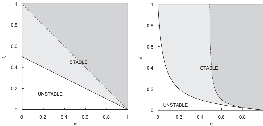
Fig. 1. Left panel: stability region for the 1-D dynamical system (30). The expected dividend yield converges to the steady state y^* = r - g only for values of (\alpha, \lambda) in the shaded area. In the darker region the convergence to y^* is monotone, whereas in the lighter region the convergence is oscillatory. Right panel: stability region for the 2-D dynamical system (28)–(29) as a function of the mutation rate \delta and memory parameter \alpha , for k = \rho/c = 10 . As in the left panel, the solid line marks the border of the stability region, while the dotted line marks the border of the region where the convergence of the expected dividend yield to y^* is monotone (darker region) or oscillatory (lighter region).
