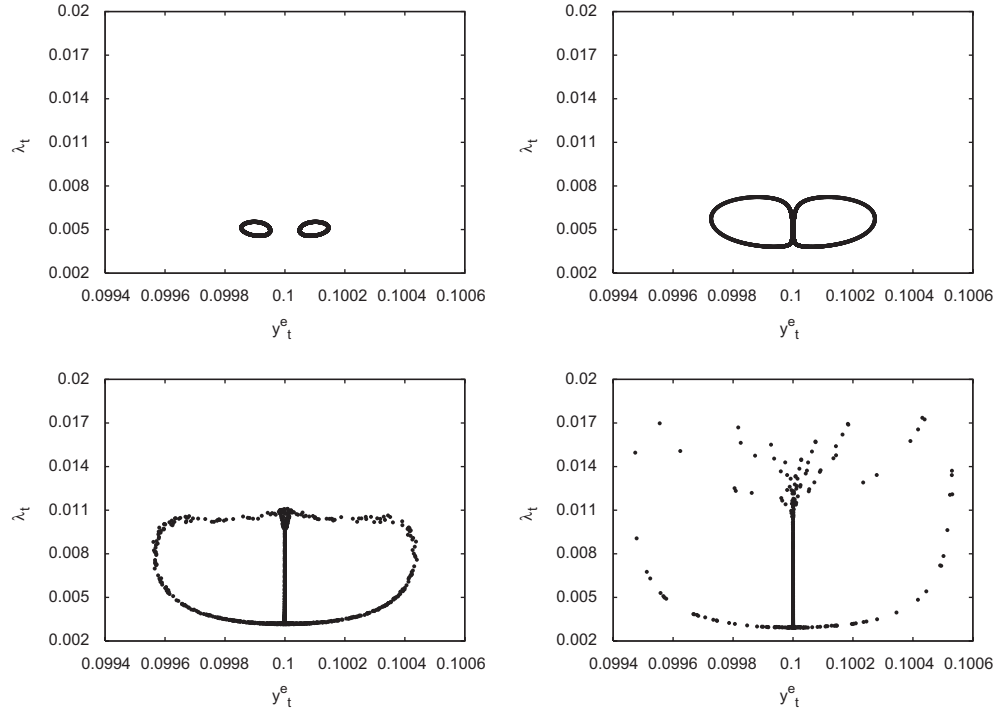
Fig. 3. Phase plots of the expected dividend yield y_t^e and the fraction of informed agents \lambda_t produced by the system of difference equations (28)–(29). Parameter values: \alpha = 0.99 , c = 0.1 , \rho = 1 (so that k = \rho/c = 10 ), r = 0.1 and g = 0 . Top left panel: \delta = 0.000675 , top right panel: \delta = 0.00066 . Bottom left panel: \delta = 0.000625 , bottom right panel: \delta = 0.000575 .
