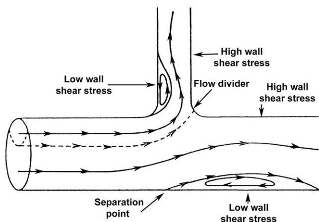
Fig. 2 Variations in flow at a 90^\circ T-junction. The stream lines shown in the diagram were videorecorded in an experimental model in glass filled with an aqueous glycerol solution containing polystyrene microspheres (50 \mu\text{m} in diameter). The dotted lines show separation flows at the point where the collateral vessel arises from the main vessel. The flow divider generates stationary recirculation flow on the side opposite to the branching vessel and on the side opposite to the main branch. In the diagram, the points along the vessel wall where shear stress is increased or decreased are shown. (Adapted with permission from Karino T, Motomiya M, Goldsmith HL. J Biomech 1990;23:537.).
