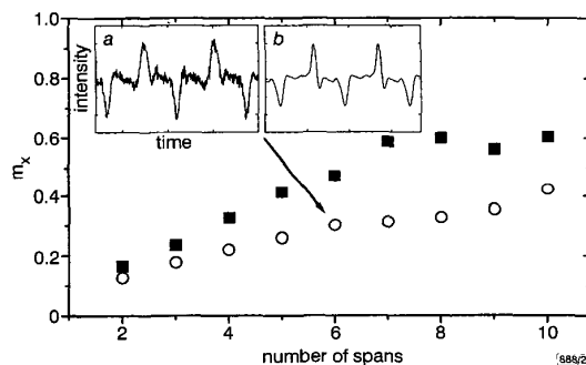
Fig. 2 Length dependence of XPM-induced distortion m_x in exactly compensated links
