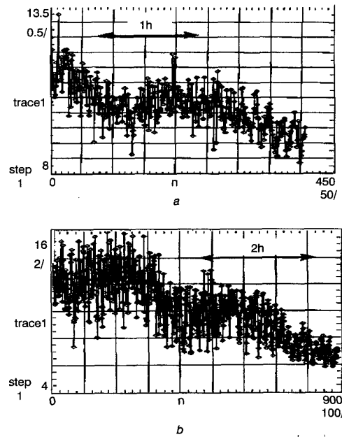
Fig. 3 Q -measurements obtained at different times at 500km and 1549nm (0.14ps/nm/km) and 1550nm (0.2ps/nm/km)
