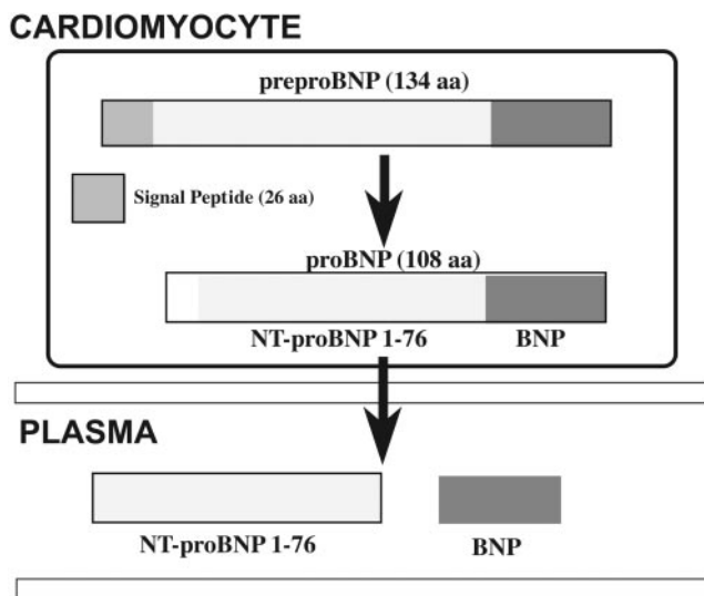
Fig. 2. Schematic representation of production/secretion pathways of BNP and of its precursor peptides.
