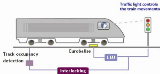
Figure 2. ERTMS Level 1.
