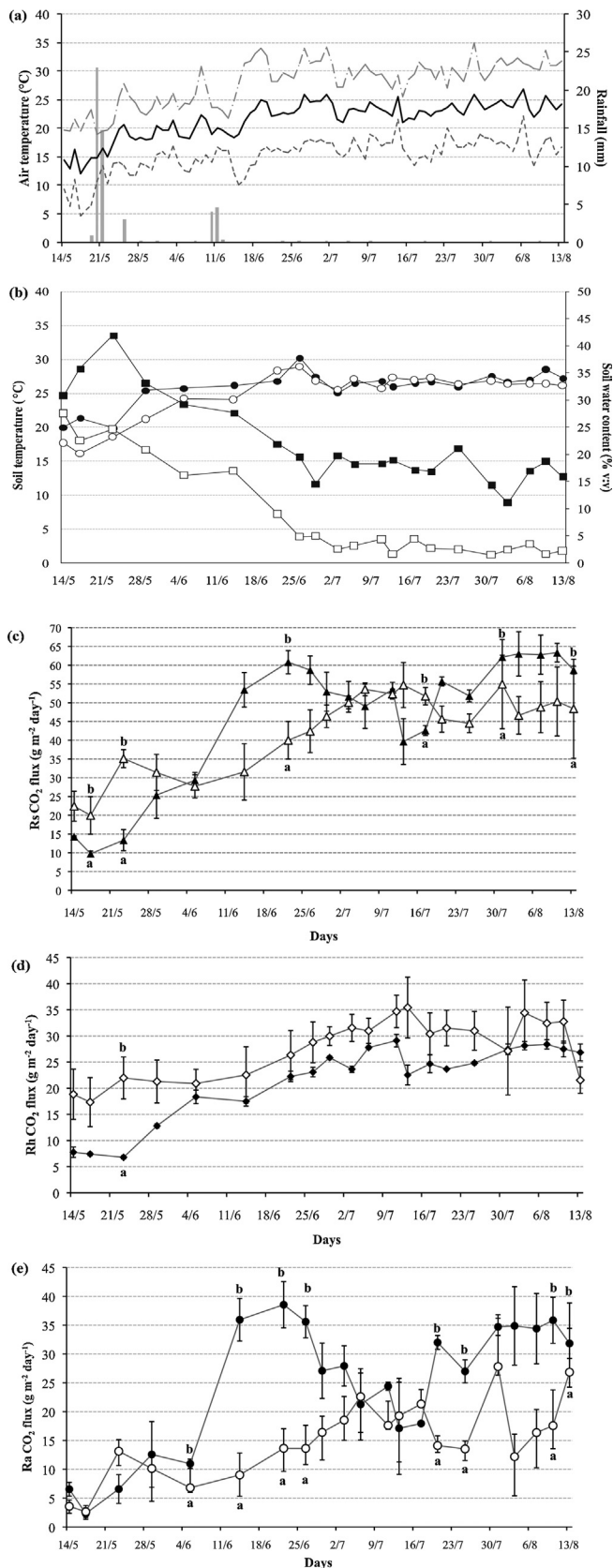
Fig. 3. Daily maximum, mean and minimum temperatures ( ^{\circ}\text{C} ) and total rainfall (mm) over the monitoring campaign (a). Mean soil temperature ( ^{\circ}\text{C} ) (shown as circle) and moisture (%; v:v) (shown as square) of agricultural abandoned peaty soils (open symbols; Aband) and a maize cultivation (filled symbols; Cult) (b). Soil temperature and moisture were measured outside the six blocks (see Fig. S1) used during the \text{CO}_2 flux monitoring campaign. Two components of the soil \text{CO}_2 fluxes,
