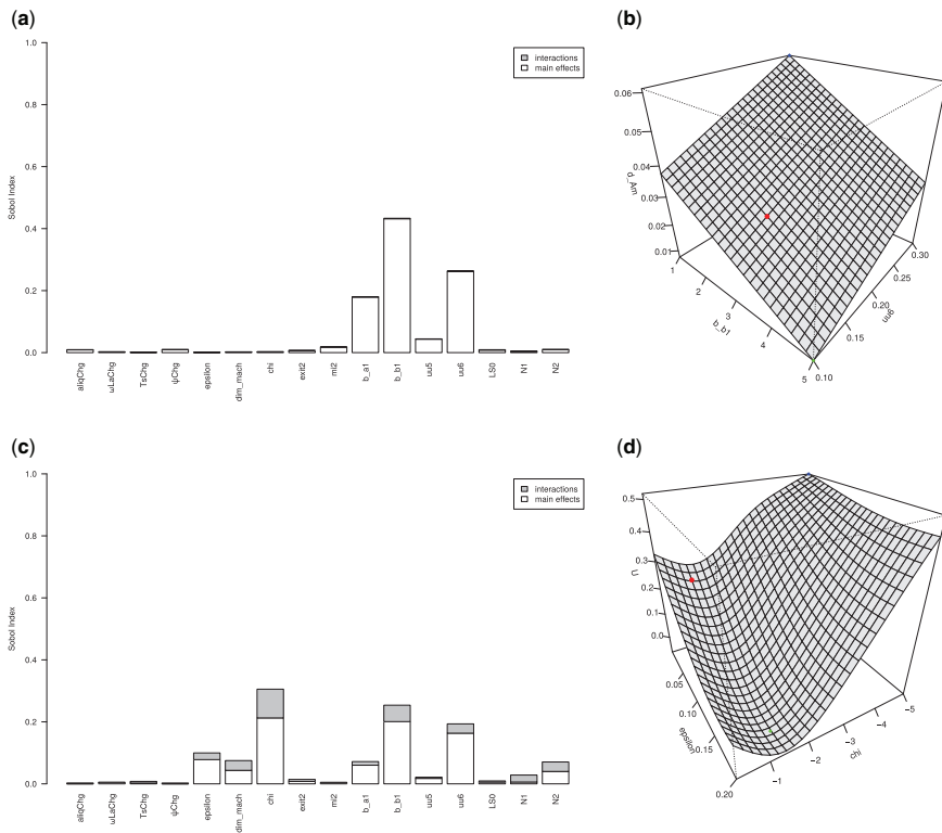
Figure 9 Global Sensitivity Analysis (continued): Competitive 2 alternative scenario. (a) Sobol decomposition: productivity growth rate. (b) Productivity growth rate (z) vs. Beta shape parameter b_{b_1} (x) and Beta distribution upper support uu_6 (y) (red dot at calibration and markers at max./min.). (c) Sobol decomposition: unemployment rate. (d) Unemployment rate (z) vs. wage increase required for labour mobility \epsilon (x) and replicator dynamics intensity -\chi (y) (red dot at calibration and markers at max./min.).
