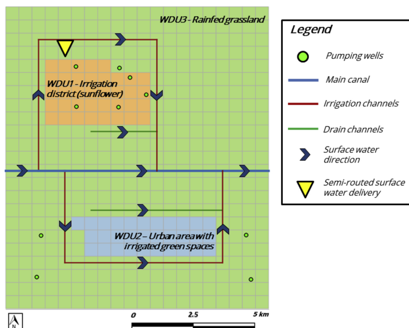
Fig. 5. Spatial distribution of WDUs and crops. The semi-routed surface water delivery to the irrigation district and the pumping wells are displayed as well.
