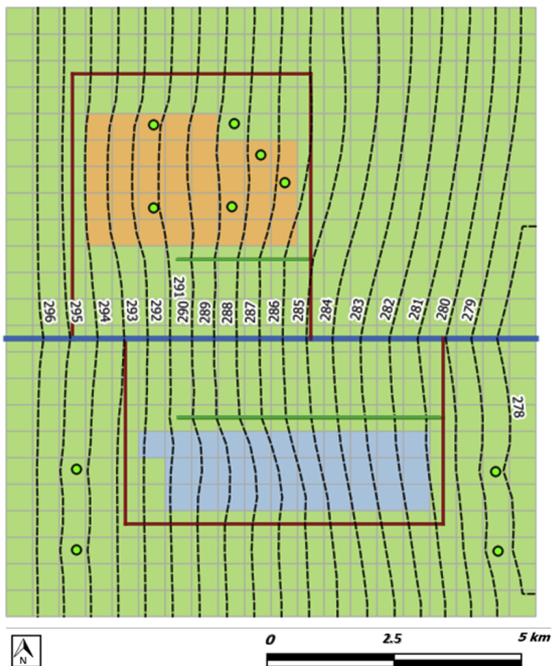
Fig. 8. Groundwater head distribution simulated on June 28 th , 2017.
