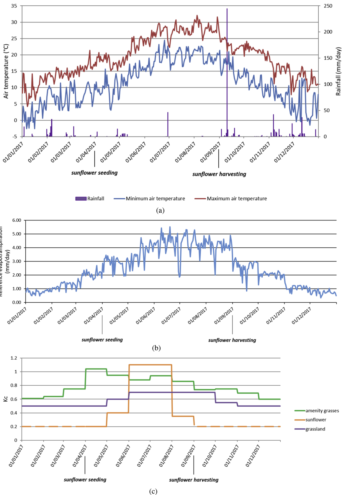
Fig. 7. (a) Climate data input for the FMP and for the CGM models. (b) Reference evapotranspiration calculated with the Hargreaves equation and input for the FMP scenario. (c) K_c values input for the three crops for the FMP scenario. The dotted, orange line refers to K_c values used to simulate evaporation from bare soil at WDU1 grid cells.
