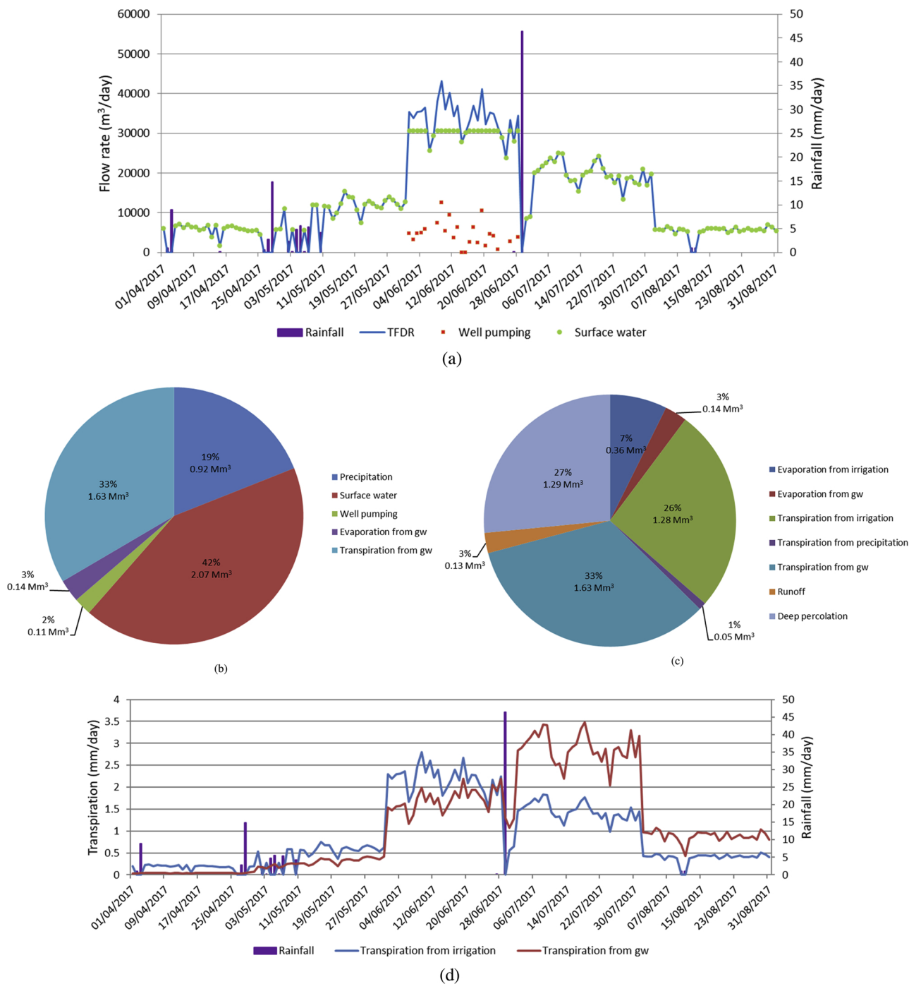
Fig. 9. (a) Demand and supply components for the irrigation district over the cropping season. (b) Inflow terms of the cumulated water balance of WDU1 over the cropping season. (c) Outflow terms of the cumulated water balance of WDU1 over the cropping season. (d) Simulated transpiration values from irrigation and from groundwater over the cropping season.
