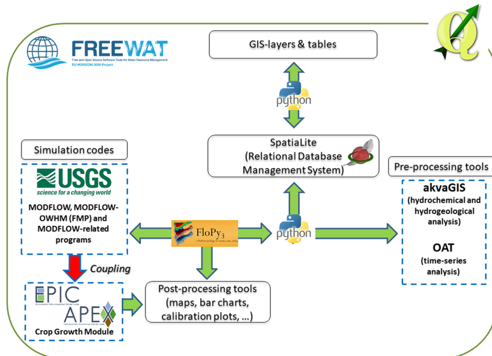
Fig. 1. FREEWAT architecture and integration of FMP and CGM within the FREEWAT platform (modified after De Filippis et al., 2017 and Rossetto et al., 2018).
