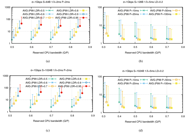
Figure 4. Experimental response-time statistics (on the Y-axes, in ms ), where vertical segments connect the average and 99^{th} percentile for each configuration: with fixed reservation period but varying reserved CPU bandwidth (on the X-axis) and workload ratio (different curves) in plots (a) and (c) on the left; with fixed CPU load but varying reserved CPU bandwidth (X-axis) and reservation period (different curves) in plots (b) and (d) on the right.
