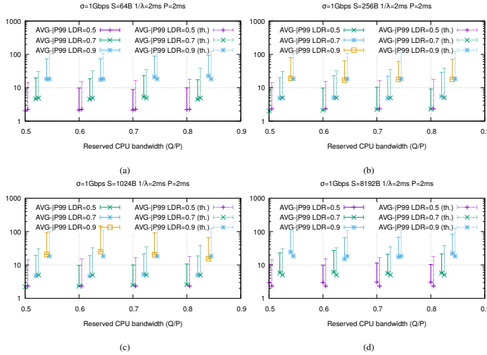
Figure 5. Experimental response-time statistics (on the Y-axes, in \mu s ) versus theoretical expectations, where vertical segments connect the average and 99 th percentile for each configuration, with different plots representing results for different packet sizes, at varying reserved CPU bandwidth (X-axis) and for various computational workload ratio (LDR) (different curves).
