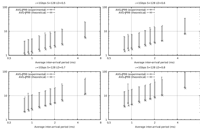
Figure 3. Experimental response times (in ms ) for various configurations, compared with the theoretical expectations (negligible sending time case). Segments connect average to the 99^{th} percentile of response-time distributions.
