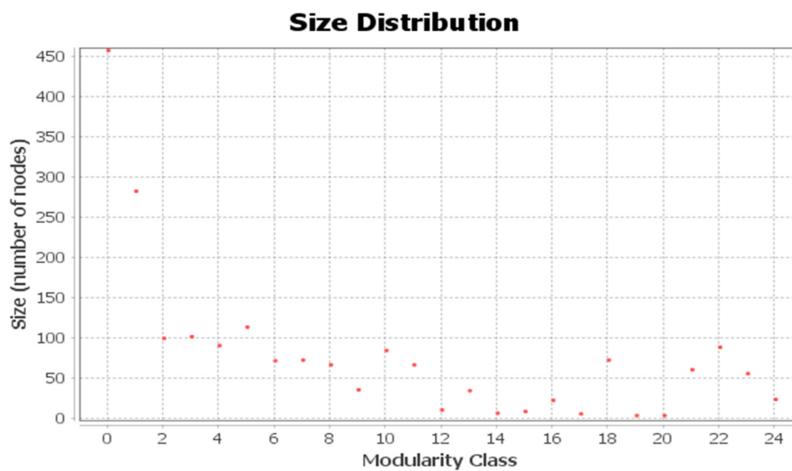
Figure A6. Community size distribution.
