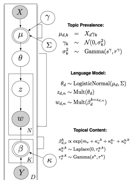
Figure A2. Structural topic modeling, in plate notation, in: (Roberts ME, Stewart BM, Tingley D, Airoidi EM. The structural topic model and Applied Social Science 2013).
