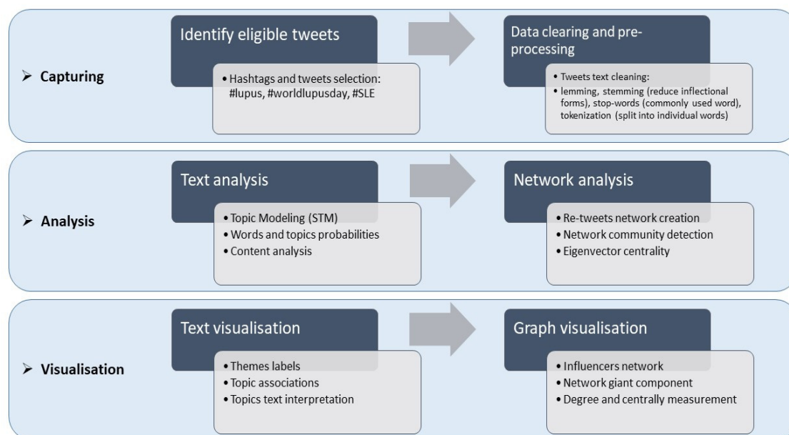
Figure 1. Framework workflow of social media Twitter analysis.
