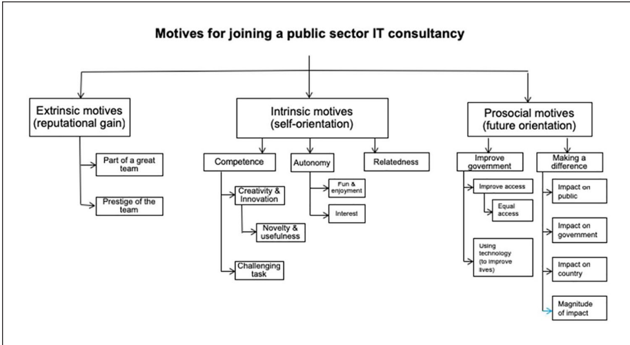
Figure 1. Coding taxonomy.
